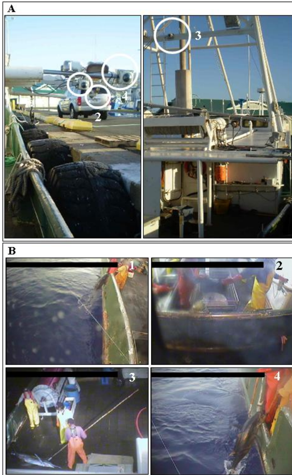
Figure 8. A. Camera installations on the deep-set vessel (D1), one on the fabricated outboard mount giving a close-up view of the waterside of the sea door and two on an existing light support covering both sides of the rail and gear handling (left). A fourth camera is on a mast support covering the deck inside the sea door (right). B. Example images from the corresponding camera views.
