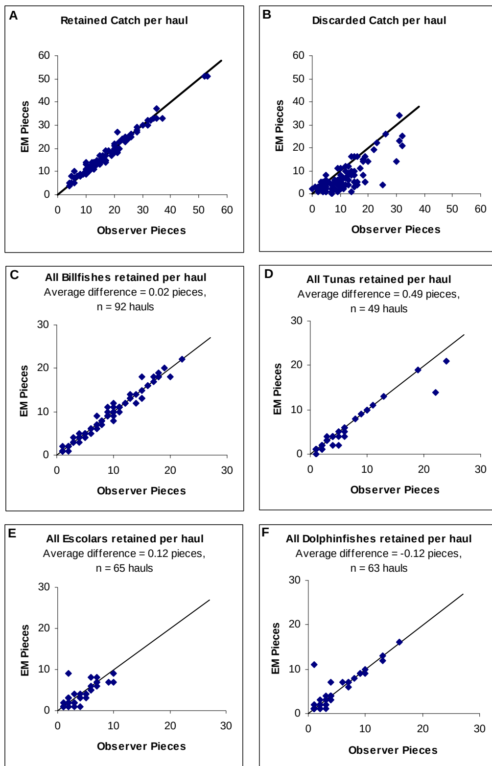
Figure 13. A-B. Scatter plots of observer versus EM retained and discarded catch per haul, respectively. C-F. Observer versus EM retained catch per haul for selected species.
