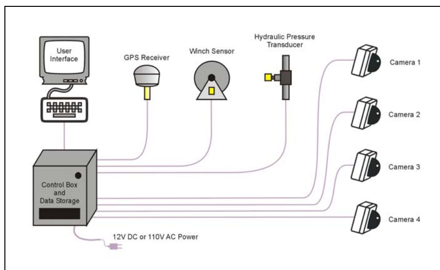
Figure 1. Schematic of standard EM system.
