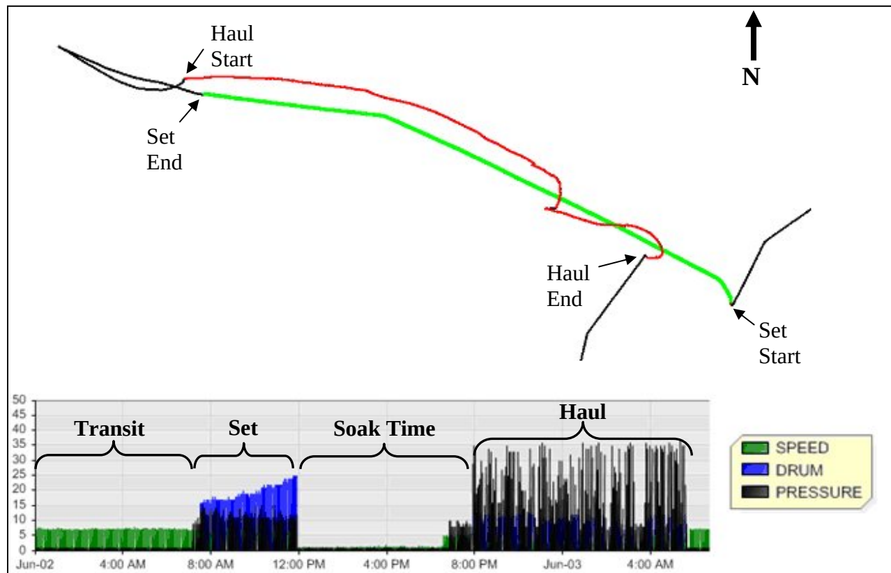
Figure 9. Example of sensor data from one of the project vessels showing sensor data representation for a set and its associated haul. The time series graphs (lower) show vessel speed (knots), hydraulic pressure (psi), and winch rotation (average counts per minute). Setting activity is associated to high drum rotation counts, low hydraulic pressure, and constant speed. Hauling is associated with high hydraulic pressure, and relatively low winch counts and speed. The spatial plot (upper) shows the vessel's cruise track for the same period, with setting highlighted in green and hauling in red.
