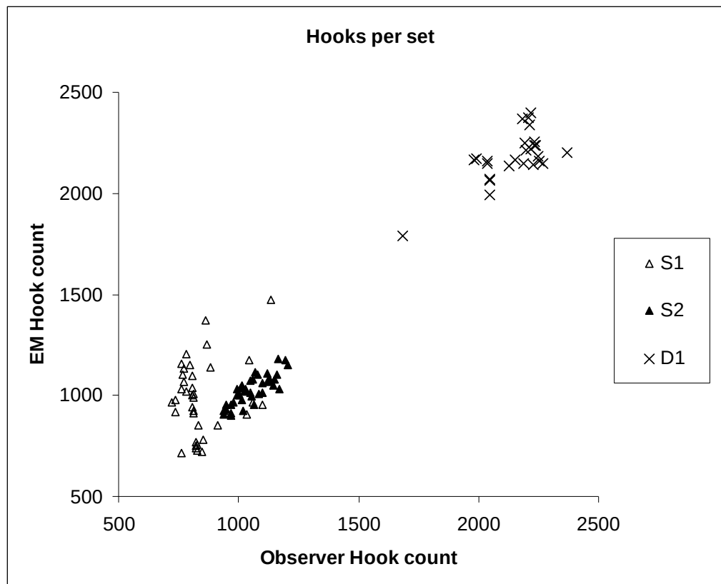
Figure 11. Scatter plot of total hook counts by observer and EM methods per haul. Comparison of EM and Observer Protected Species Interactions
